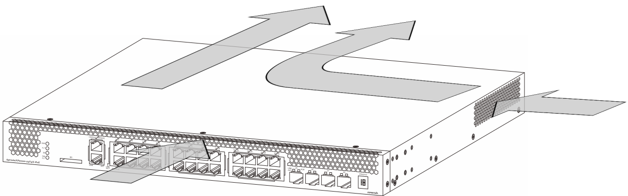
図 3-6 ApresiaNP2100-24T4X-PoE、ApresiaNP2100-48T4X-PoE、ApresiaNP2000-24T4X-PoE、 ApresiaNP2000-48T4X-PoE
